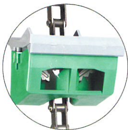
Showing high grain flow across sensor areas. Other yield sensors (shown in white) don't get an accurate reading because grain is hitting grain instead of the sensor.
